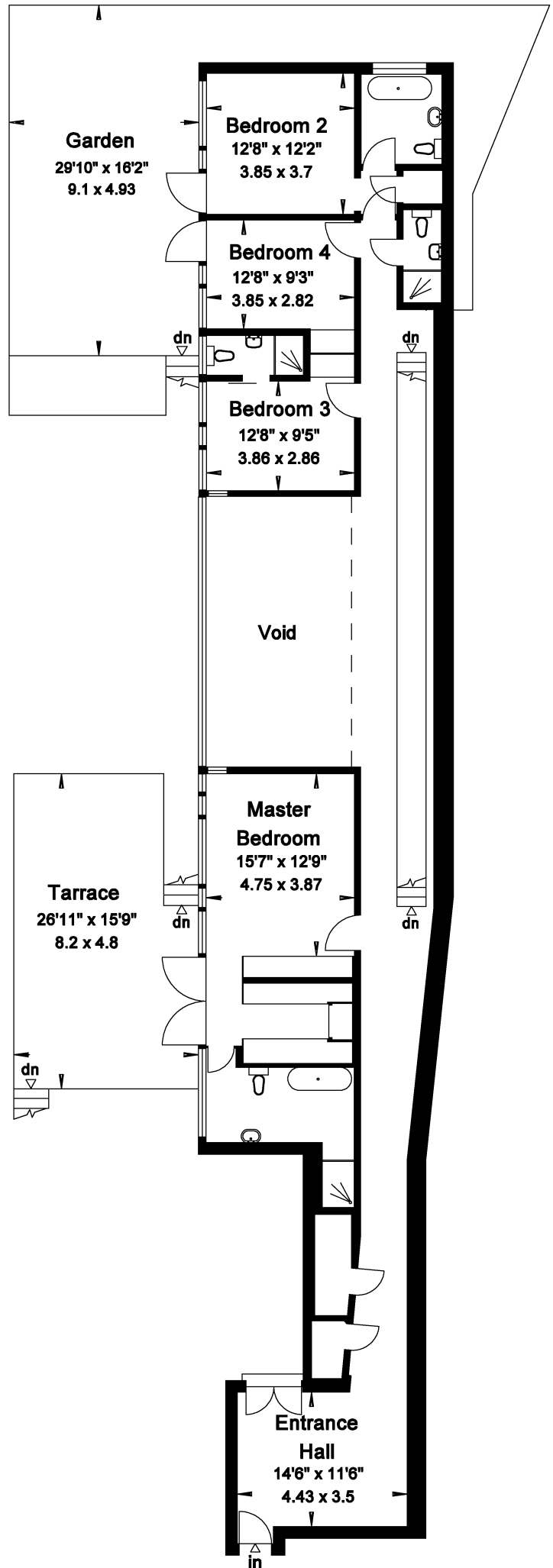
Ground Floor
